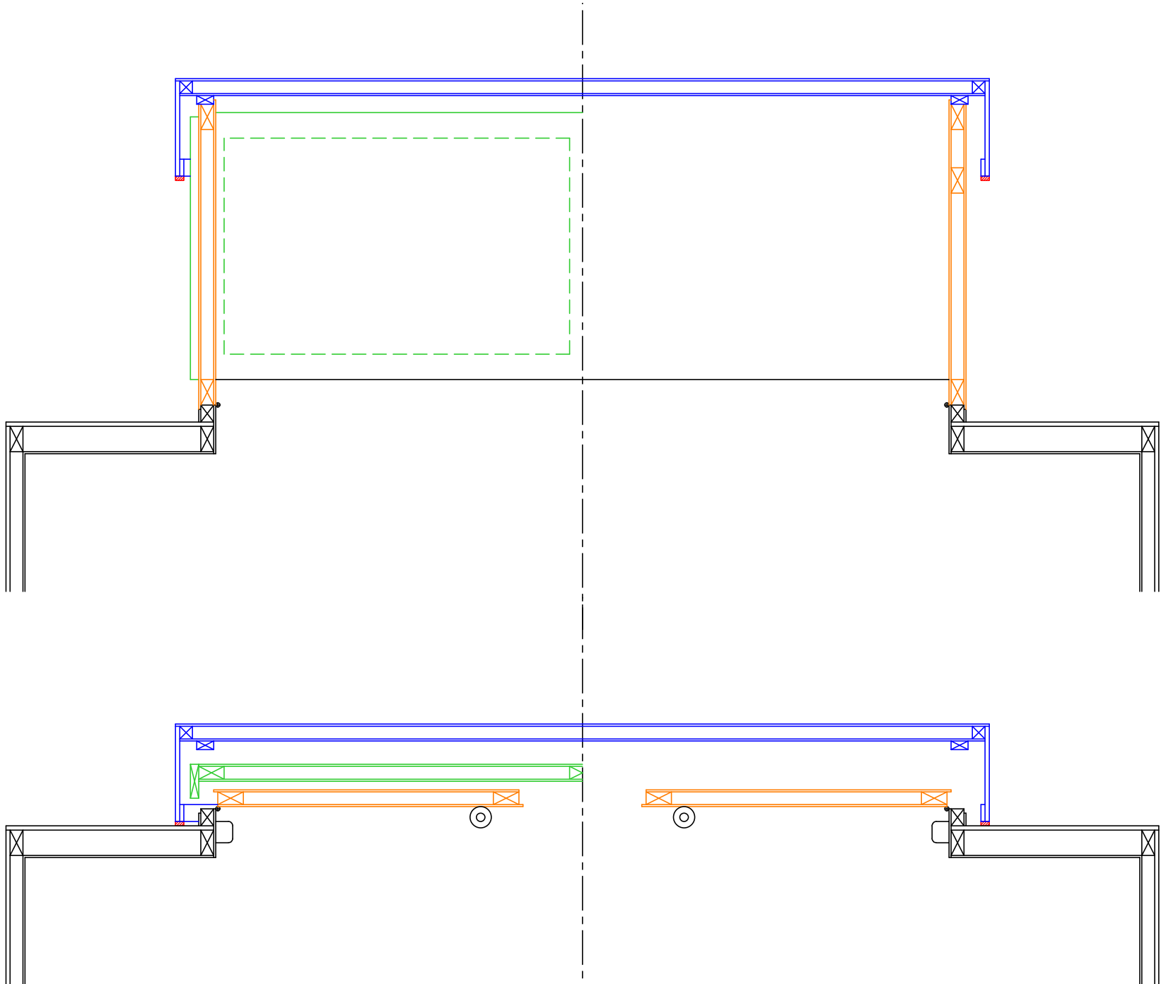
COMPACT 2 ROOF - Transverse Sections - Scale 1:8 @ Letter
